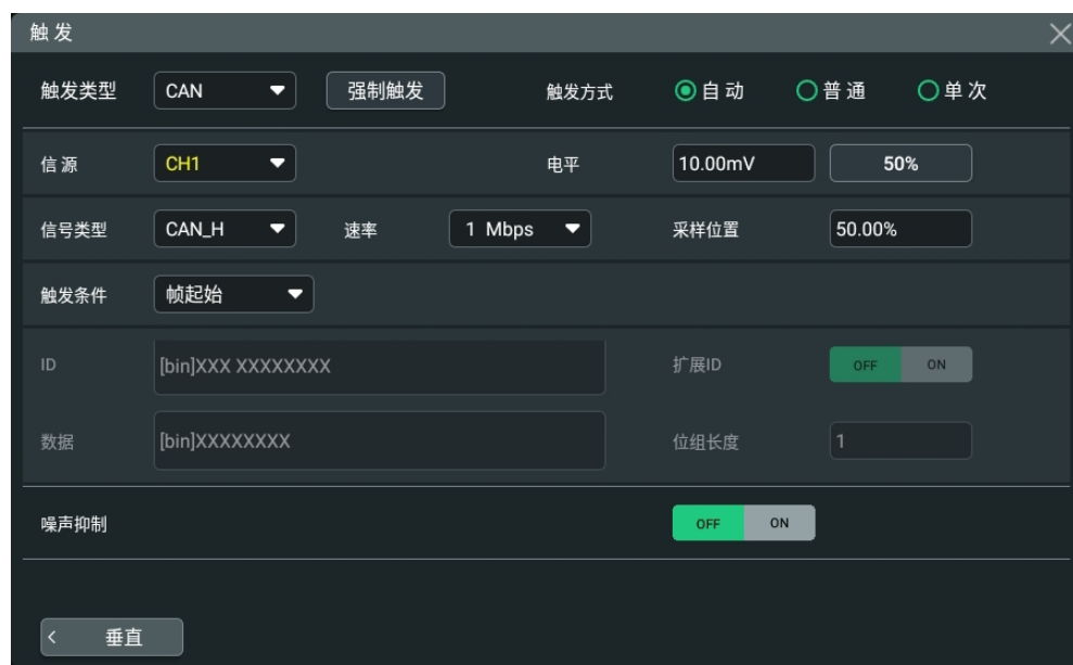
图 8.33 CAN 触发配置菜单
